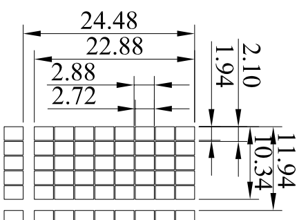
DOTS DETAIL 5:1
